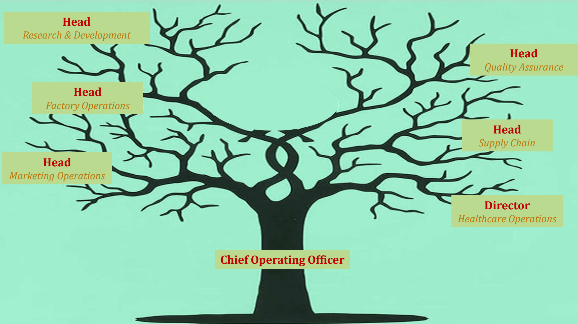
Signature Tree
